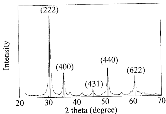
Fig. 3. X-ray diffraction of dried and annealed nanoscaled, crystalline \text{In}_2\text{O}_3:\text{Sn} powder prepared by a controlled growth reaction at atmospheric pressure. The vertical lines correspond to the data of the JCPDS database, Table 06-416 (cubic indiumoxide structure).
