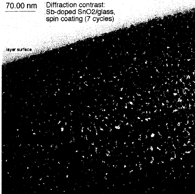
Fig. 11. Cross-section of a multilayer \text{SnO}_2 :Sb coating deposited by spin coating on a glass substrate with a particulate sol having a solid content of 7.7 Vol.%. Each layer was sintered in air at 550^\circ\text{C} during 15 min.
