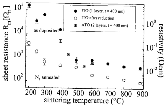
Fig. 8. Sheet resistance (left) and resistivity (right) of 400 nm thick ATO and ITO coatings versus sintering temperature for a sintering time of 30 min. The ITO coatings were annealed afterwards in a nitrogen atmosphere at 300^\circ\text{C} .
