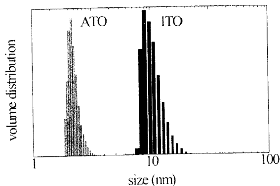
Fig. 5. ATO and ITO hydrodynamic particle size distribution in the suspension.
