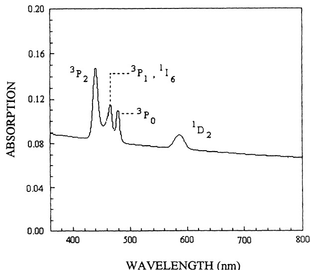
FIG. 1. Absorption spectrum of \text{Pr}^{3+} in fluoroindate glass at room temperature (sample with x=0.2 ).
