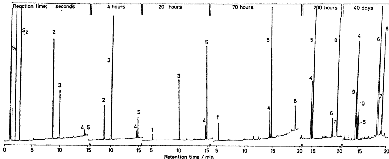
FIGURE 3 Chromatograms taken during Amberlyst treatment of Q_6L_6 : dodec methylpentasiloxane internal standard peak ( S_1 ); n-tetradecane internal standard peak ( S_2 ); Q_2L_6 (1); Q_6L_6 (2); Q_6L_8 (3); Q_6L_{10} (I) (4); Q_6L_{10} (II) (5); Q_6L_{12} (I) (6); Q_6L_{12} (Ia) (7); Q_6L_{12} (II) (8); Q_6L_{10} (9) and (10). Designations of Q_6L_{12} (I) and Q_6L_{12} (II) correspond to those in ref. 3. For the g.c. conditions see the text
