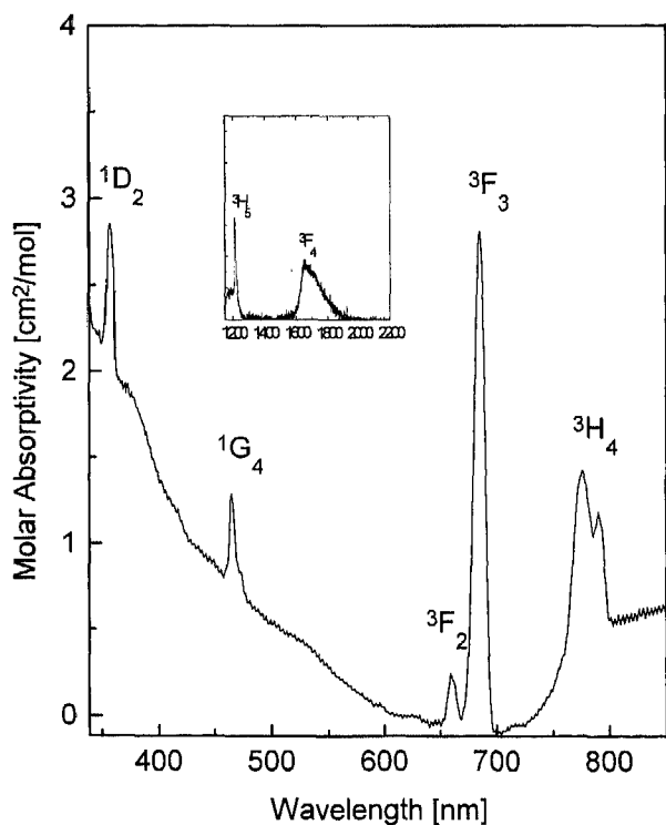
Fig. 1. Absorption spectrum of \text{Tm}^{3+} in fluoroindate glass, at room temperature, in the spectral range from 340 to 850 nm and from 1150 to 2200 nm. Sample with x=3 mol% of \text{Tm}^{3+} .
