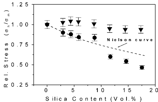
Figure 7. Tensile strength of PIHs (●) and PHIHs (▼) as a function of silica content. For comparison, theoretical curves based upon the Nielsen's theory (34) are shown.
