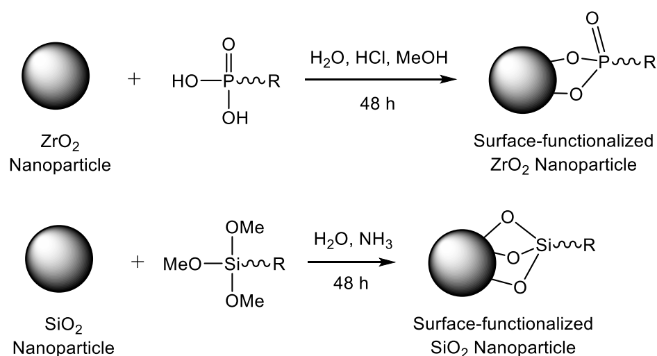
Figure 1. Surface-functionalization of the \text{ZrO}_2 and \text{SiO}_2 nanoparticles. For details see supplementary materials.
