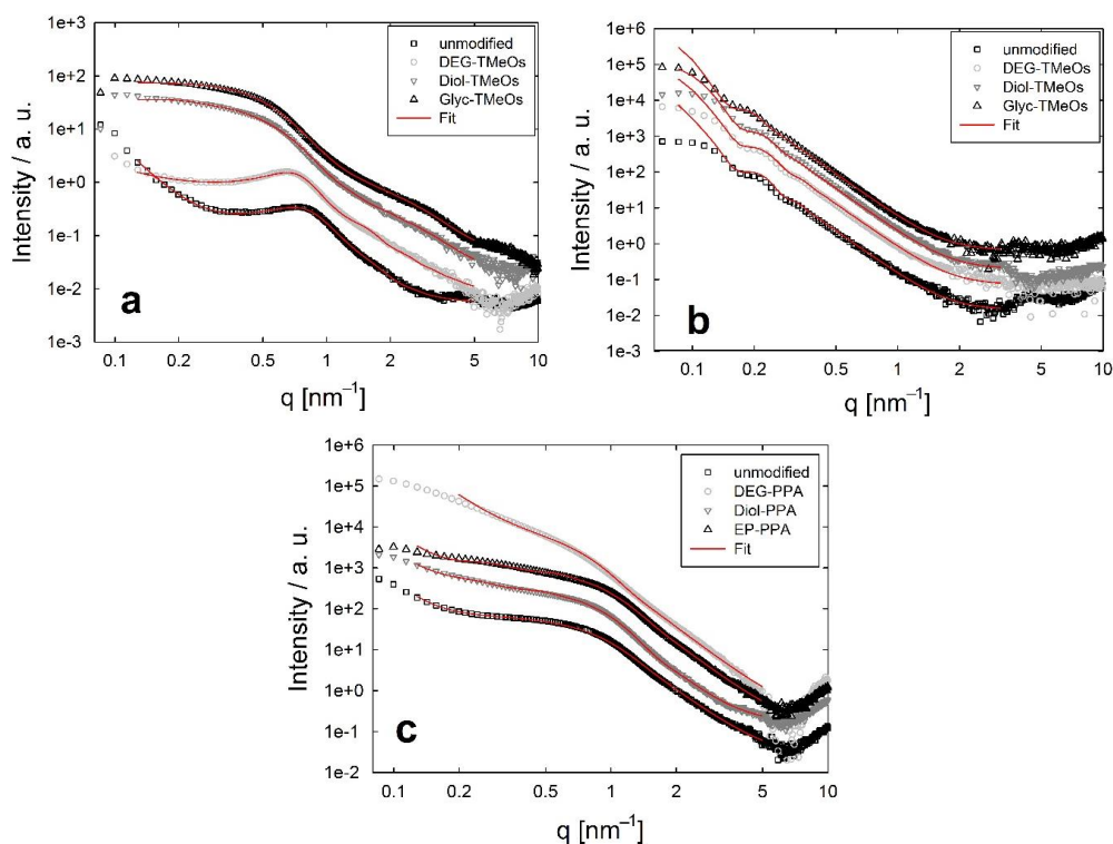
Figure 6. SAXS scattering curves, exemplarily shown for 5 wt% inorganic nanofiller content of epoxy resin nanocomposites containing (a) small SiO 2 , (b) large SiO 2 , and (c) ZrO 2 .
