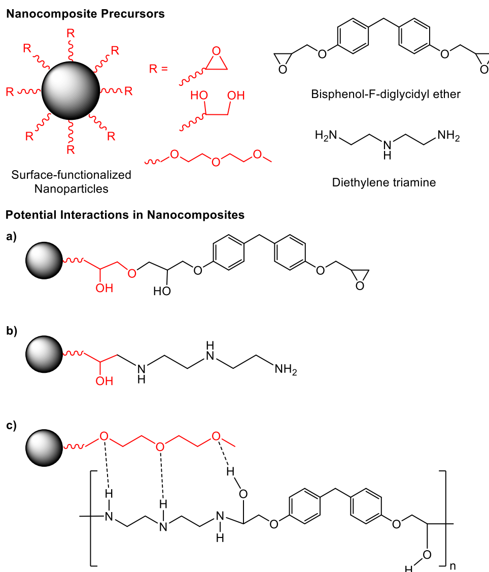
Figure 2. Potential interactions between surface-functionalized nanoparticles and epoxy resin in nanocomposites: (a) reactions between hydroxy-groups located at the nanoparticle surfaces with epoxides of the resin mixture, (b) epoxide groups from the nanoparticle surface are attacked by the hardener molecules, (c) hydrogen-bond formation between epoxy resin and ethylene oxide moieties on particle surface.
