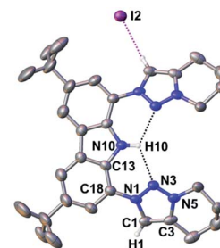
Fig. 2 Compound 3 forms intramolecular hydrogen bonds in the solid-state. Thermal ellipsoids are shown at the 50% probability level; hydrogen atoms (except the ones bonded to the carbazole's nitrogen atom and the triazolium heterocycles) are omitted for clarity. Selected bond lengths [Å], angles [°], and dihedral angle [°]: N10–H10 0.88(2), N10–C13 1.391(6), C18–N1 1.433(7), N1–N3 1.326(6), N3–N5 1.311(6), C1–C3 1.353(8), N3–H10 2.351(19), C13–N10–C13 107.0(6), N1–C1–C3 105.8(5), C13–C18–N1–N3 29.2(7).
